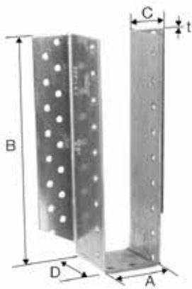
Bjelkesko type BSD
