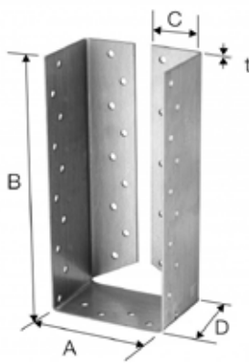
Bjelkesko type BSIL
